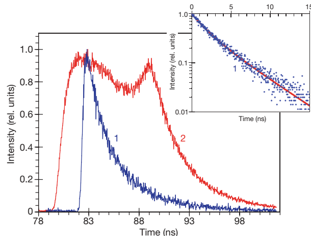
Figure 3 | Emission kinetics. Main panel, emission kinetics detected at 480 nm (1) and 520 nm (2). Inset, trace 1 plotted in semi-logarithmic coordinates (dots) and the corresponding fitting curve. The beginning of each emission kinetic trace coincides with the 90-ps pumping pulse.
